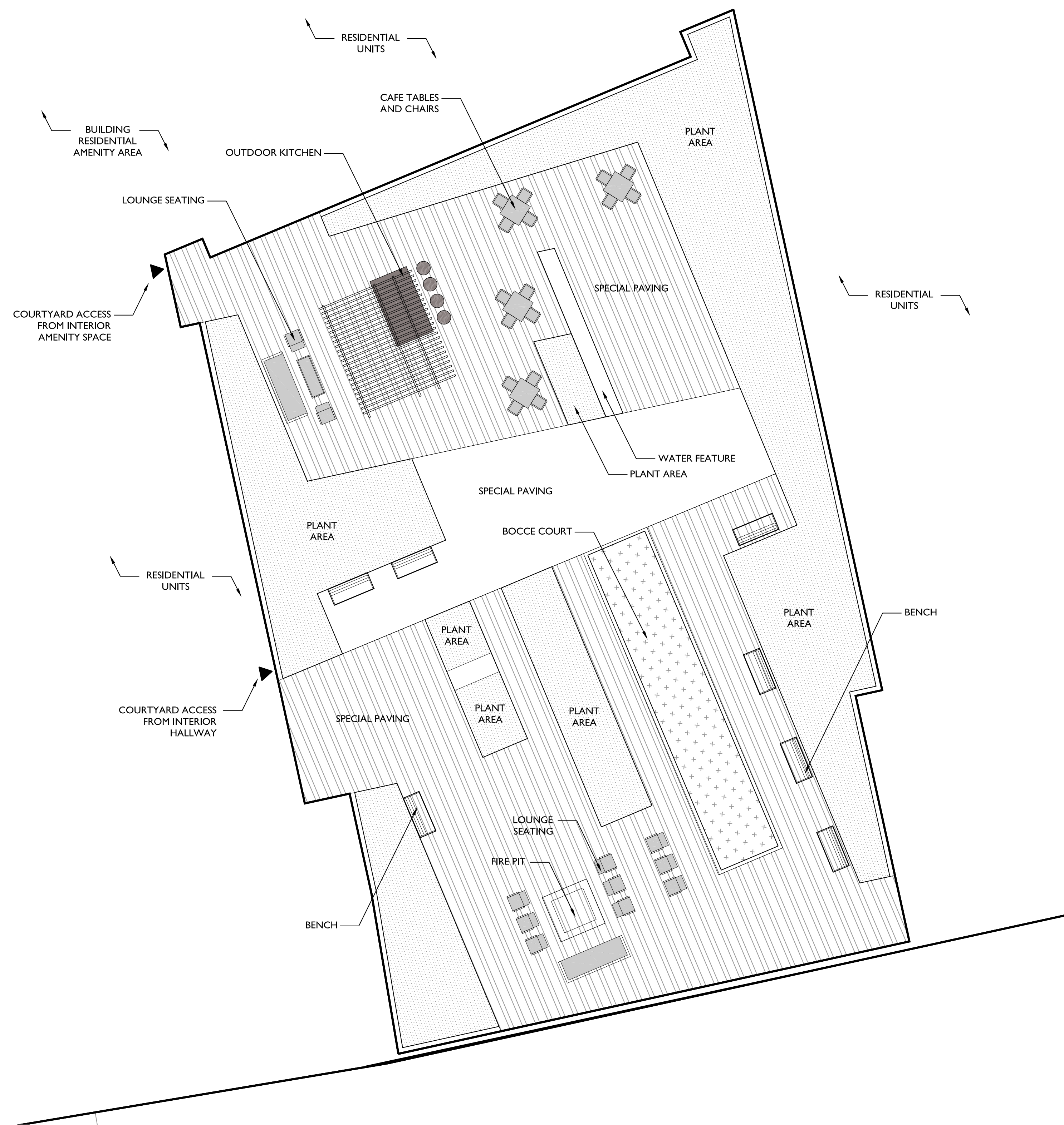
2 GARDEN COURTYARD (1ST RESIDENTIAL FLOOR ABOVE COMMERCIAL) 1" = 10' L-2.3 PLAN
