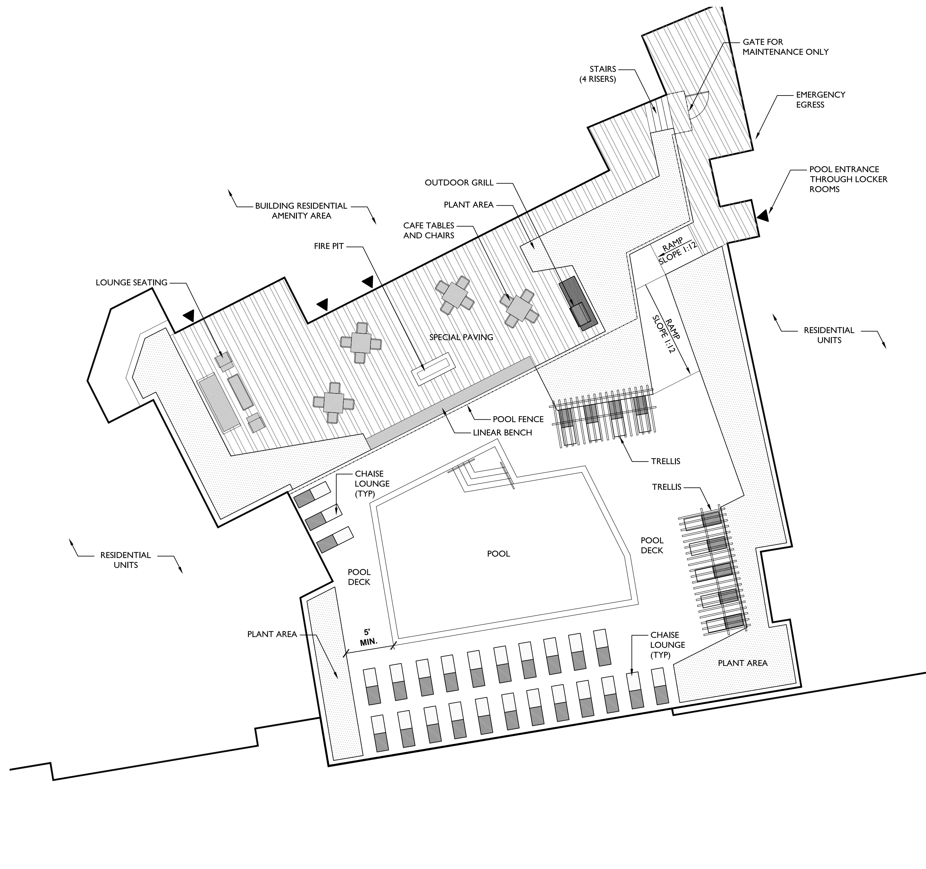
1 POOL COURTYARD (1ST RESIDENTIAL FLOOR ABOVE COMMERCIAL) 1" = 10' L-2.3 PLAN
