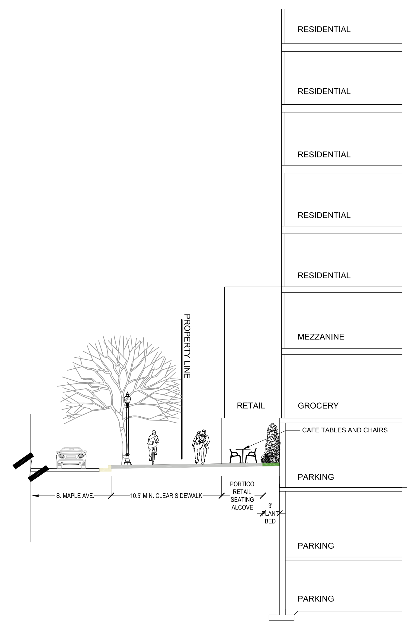
1 SECTION L-2.4 PORTICO RETAIL ON S. MAPLE AVE. 1"=10'
