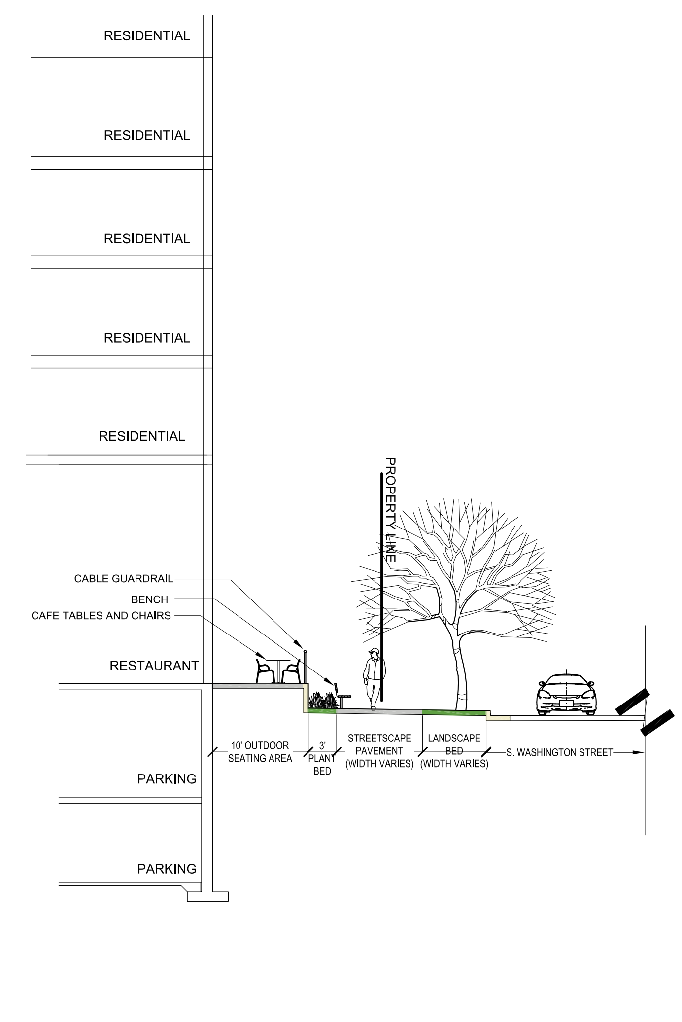
2 SECTION L-2.4 OUTDOOR DINING ON S. WASHINGTON STREET 1"=10'
