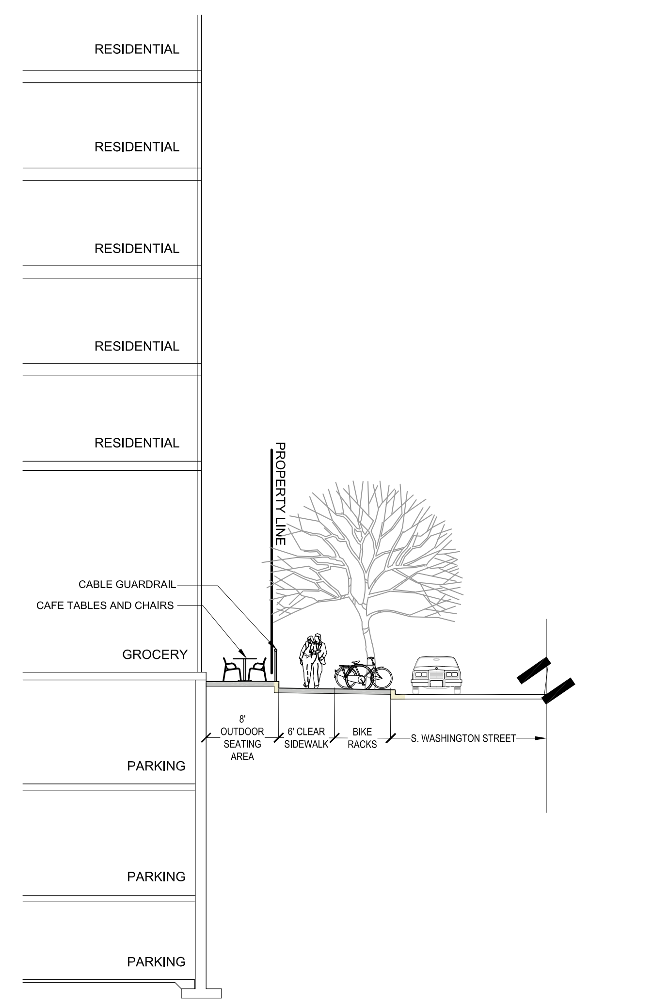
3 SECTION L-2.4 OUTDOOR DINING AT GROCERY STORE 1"=10'
