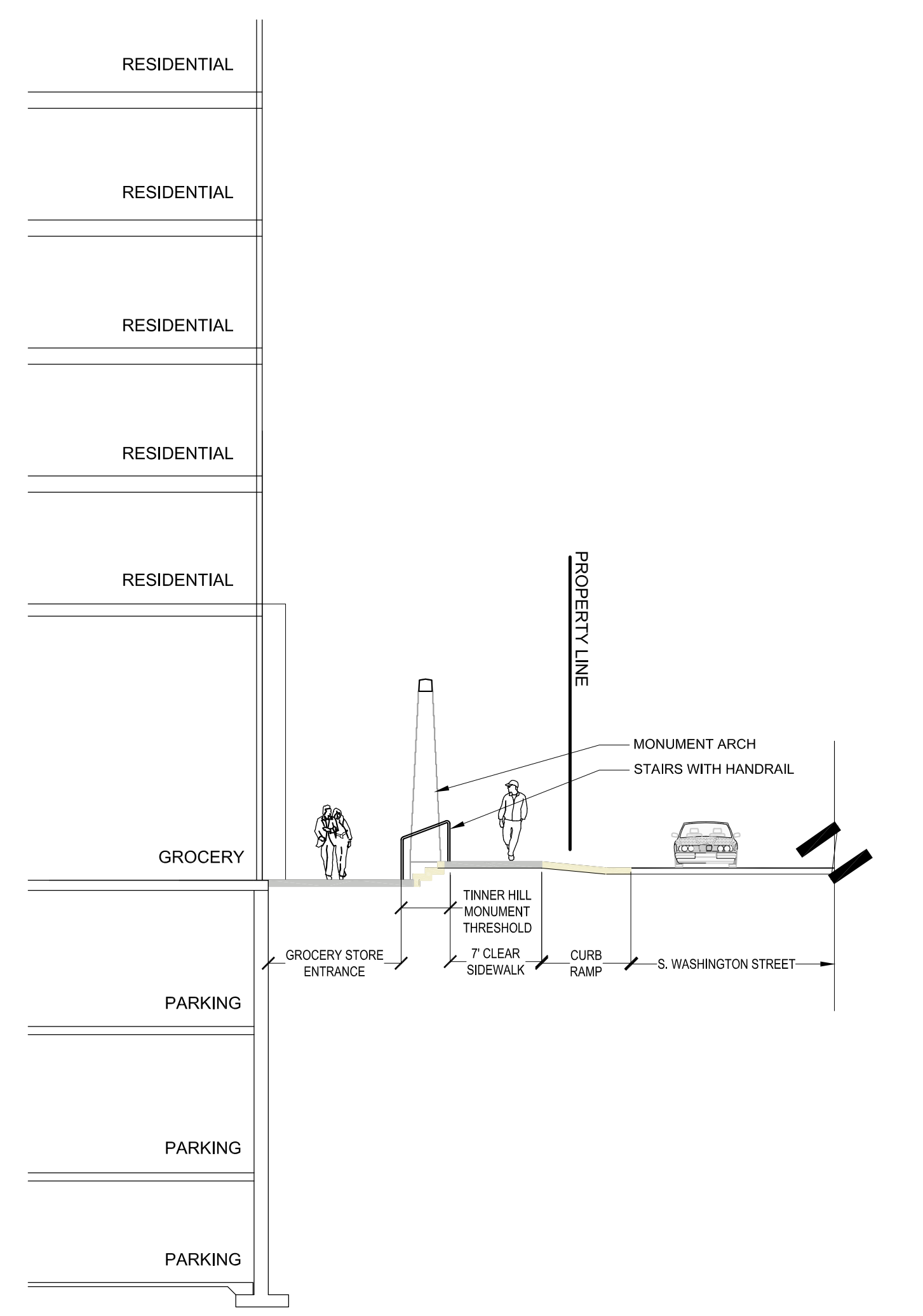
4 SECTION L-2.4 TINNER HILL MONUMENT AT GROCERY STORE ENTRANCE 1"=10'
